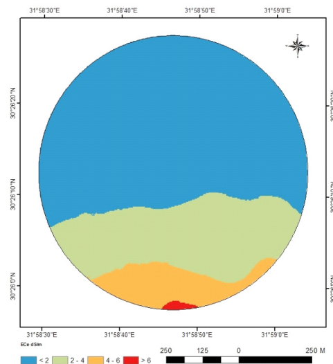
Mapped soil salinity (bulk average)
